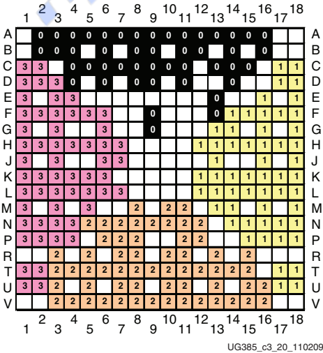
Figure 3-20: CSG324 Package—LX45 I/O Bank Diagram
