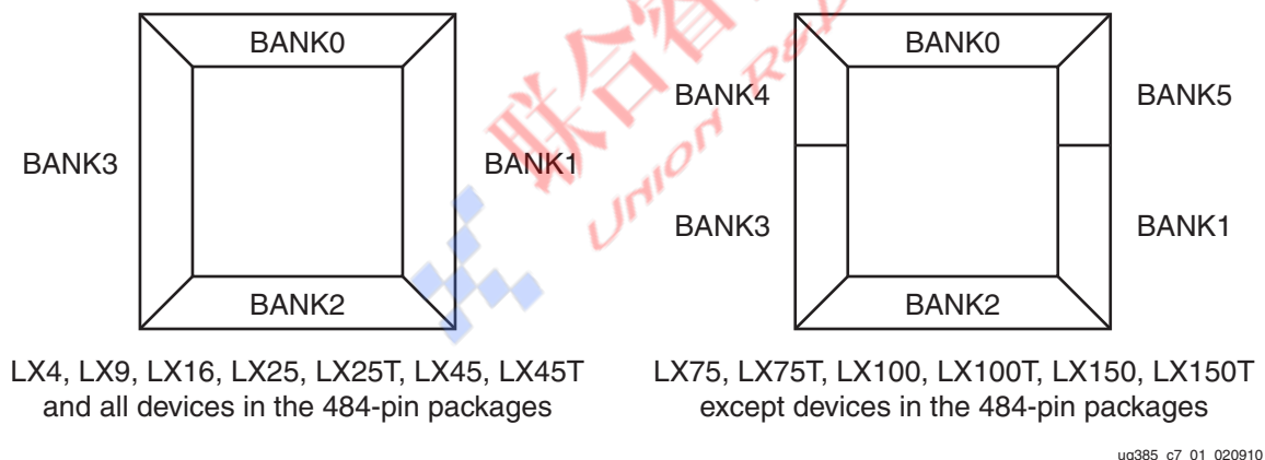
Figure 7-1: Spartan-6 FPGA I/O Bank Migration
