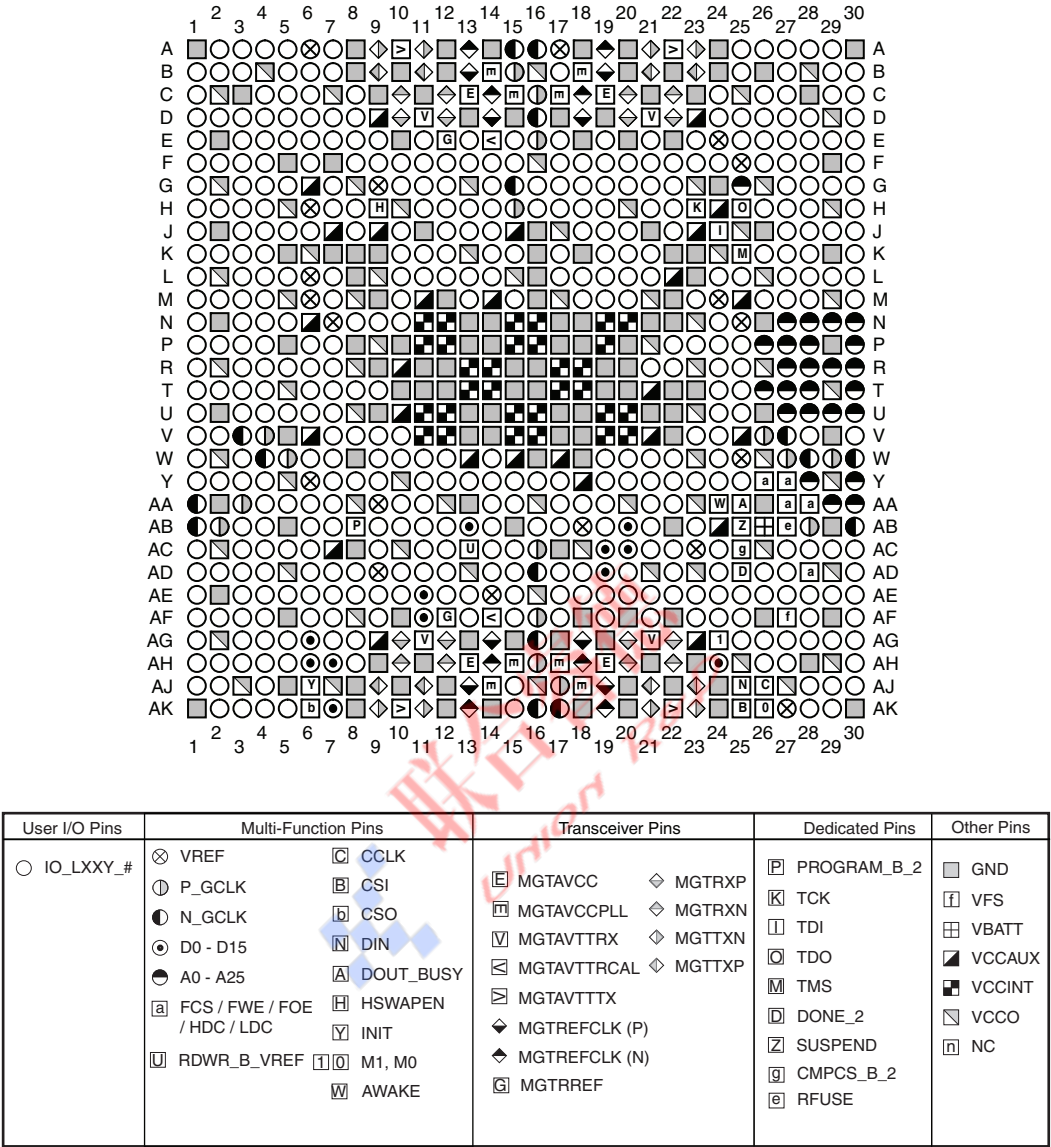
Figure 3-67: FG(G)900 Package—LX150T Pinout Diagram
