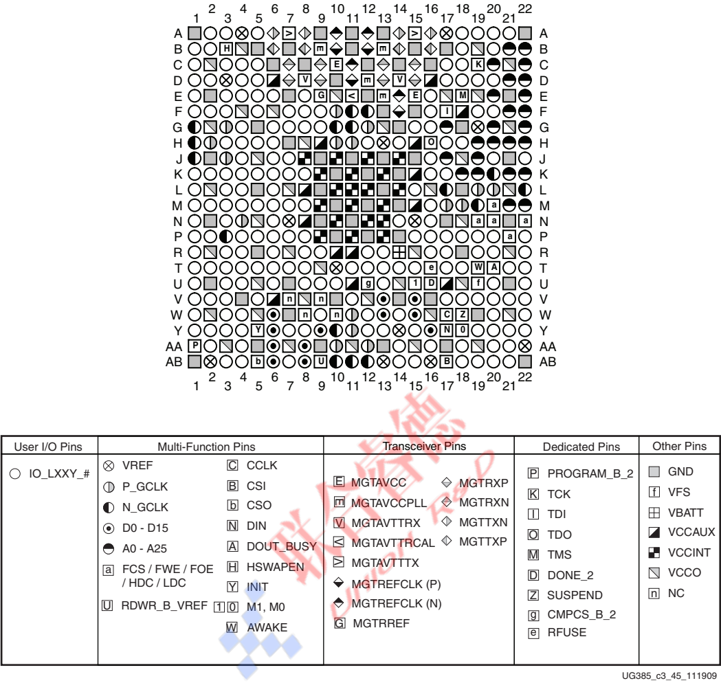
Figure 3-45: CS(G)484 Package—LX75T Pinout Diagram
