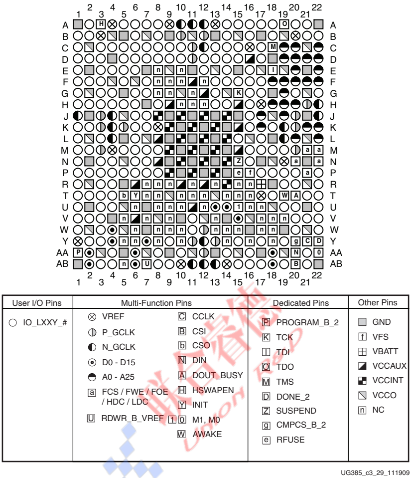
Figure 3-29: FG(G)484 Package—LX75 Pinout Diagram
