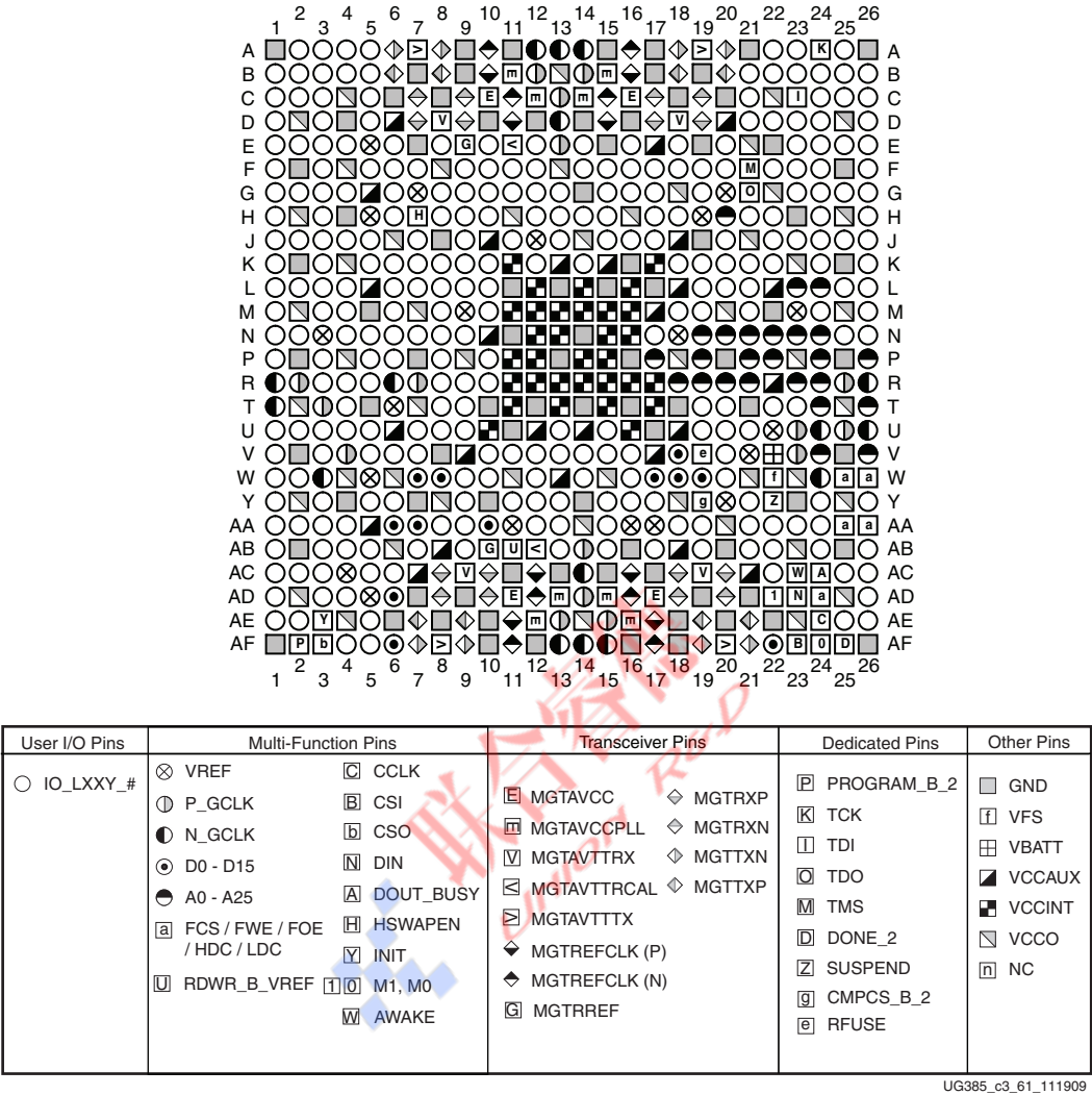
Figure 3-61: FG(G)676 Package—LX150T Pinout Diagram
